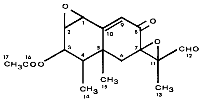
PR-Toxin
