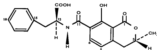
Ochratoxin B
