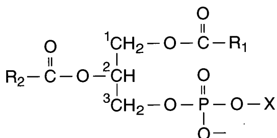
Figure 3.3. Generalized structure for a common glycerophospholipid. \text{R}_1 and \text{R}_2 represent two fatty acids, and \text{X} may be ethanolamine, choline, serine, inositol, glycerol, or phosphatidylglycerol.
