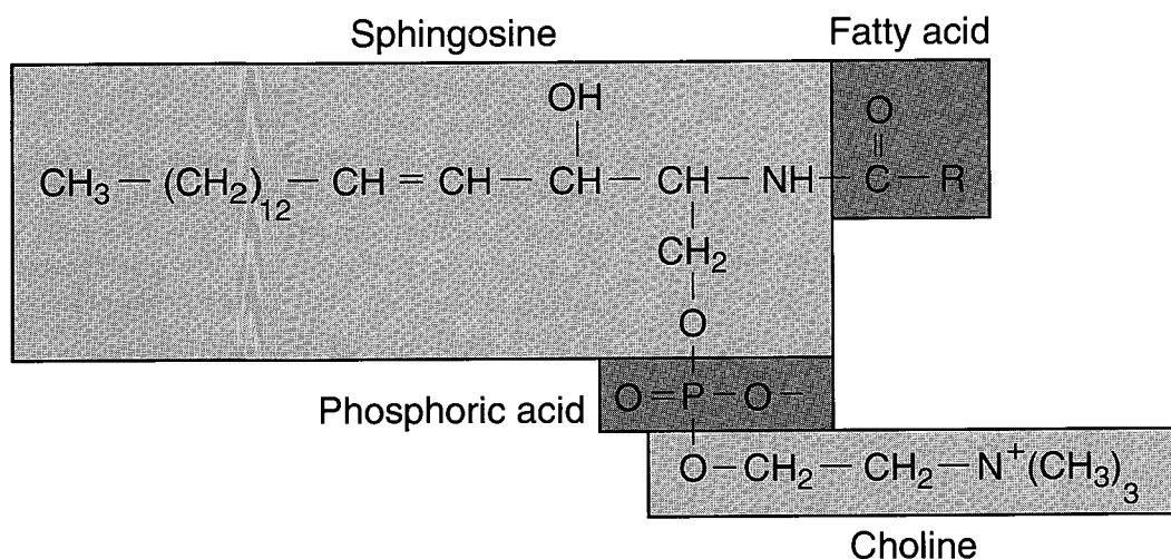
Figure 3.4. Generalized structure of a sphingophospholipid (sphingomyelin).
