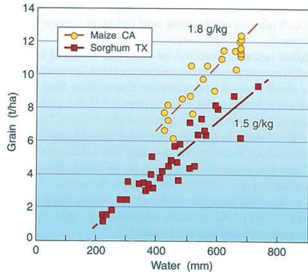
Figure 6.3.2. Relations in the field of the yields of grain to water supply in California maize and in Texas sorghum. The slopes of 1.5 and 1.8 grain/kg are 3 to 4 g biomass/kg water, respectively. Engineers and agronomists employ dimensions of kg grain/m 3 water, which give the same values numerically as the g/kg used here (Stewart et al., 1977; Stewart et al., 1983).
