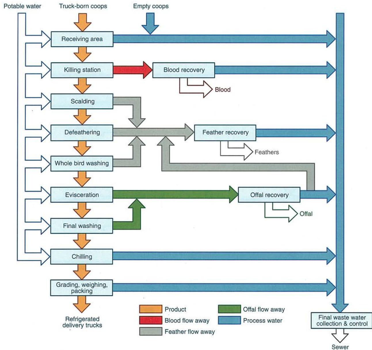
Figure 8.8. Process flow diagram for poultry processing operation
